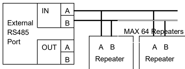
Fig. 1 The P-9957E-RP wiring diagram
